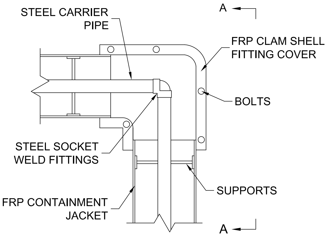
FRP CONTAINMENT ELBOW DETAIL N.T.S.
