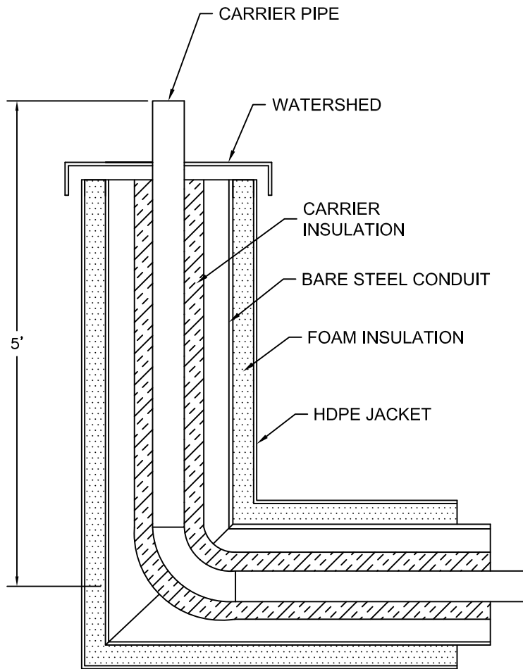
TYPICAL INSUL-800 RISER WITH WATERSHED DETAIL
